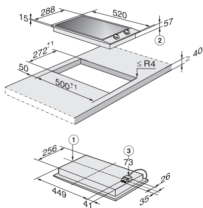
CS1212-3I, CS1212-1I (Installation drawing)
